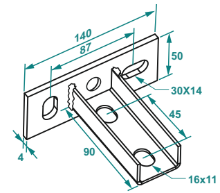
UT5 02 EG Lengthwise Model
