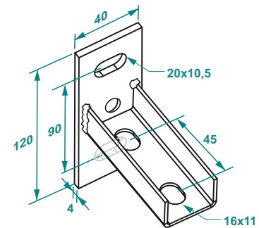
UT4 11 EG Crosswise Model
