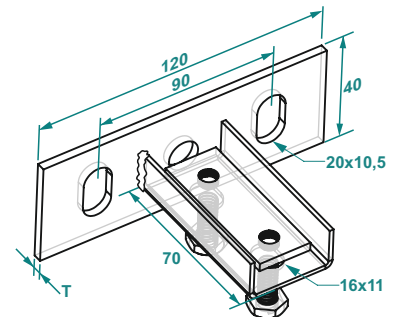
UT4 11 EG Crosswise Model
